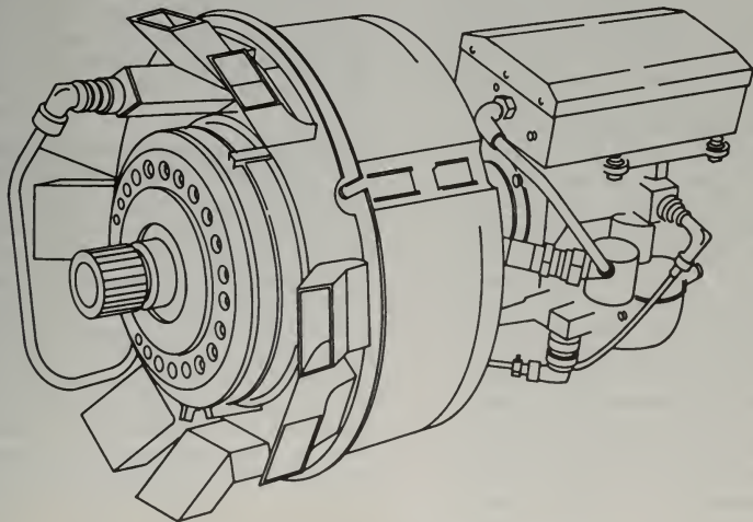
FIGURE 5-23. Fuel/air combustion starter.
